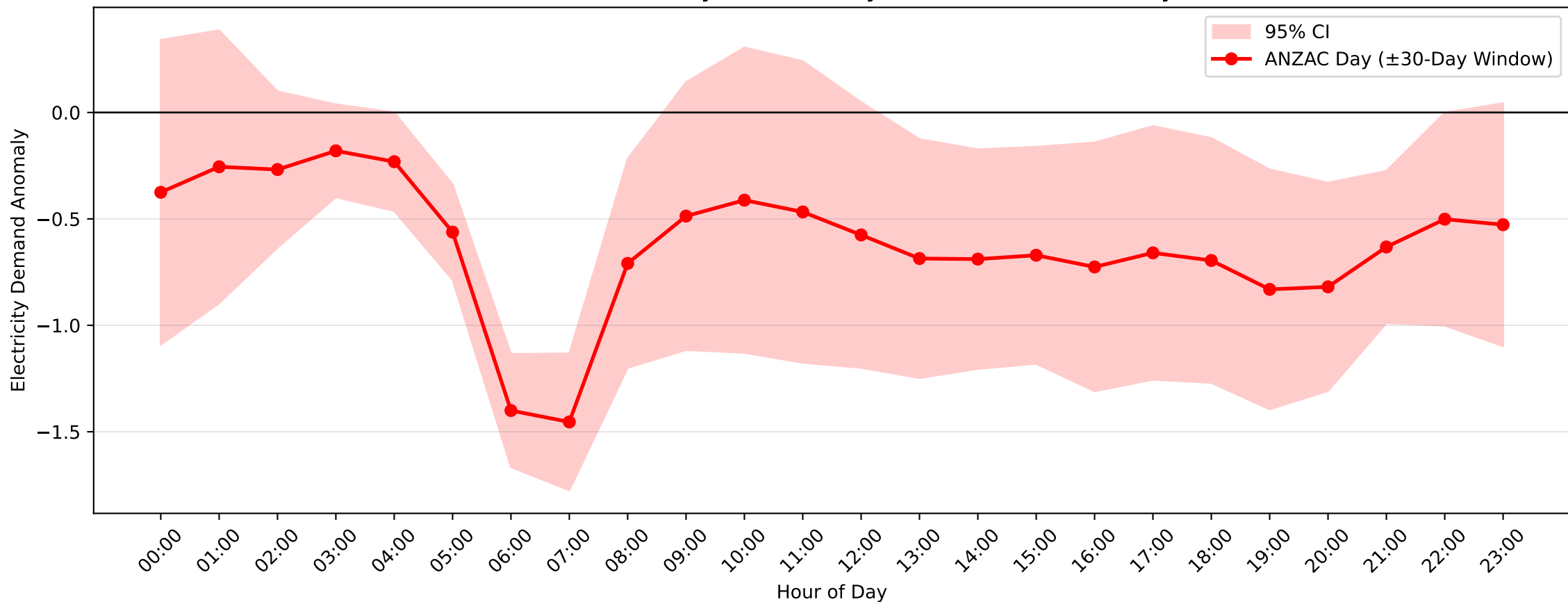
Morisset Demand Anomaly: ANZAC Day (2004–2017, \pm 30 -Day Window)
